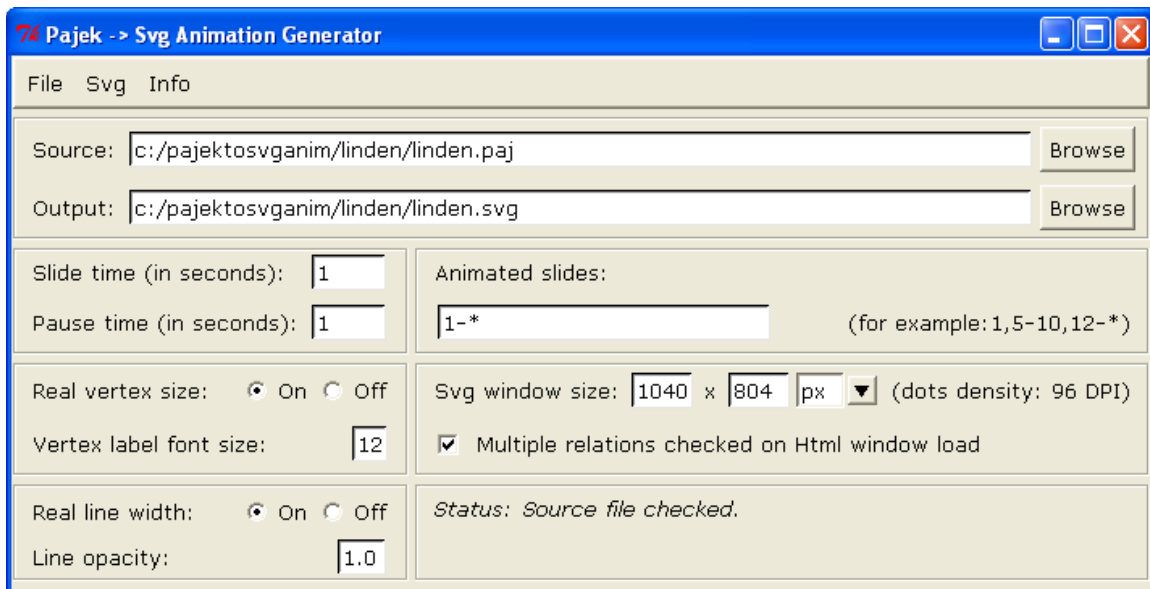
Picture 1: Input Pajek file selection in the Main window of the program PajekToSvgAnim.
